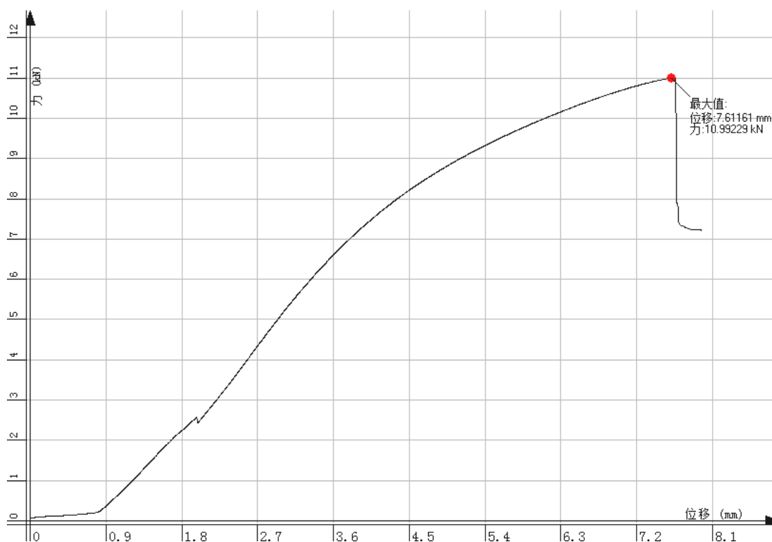
Force-displace curve
